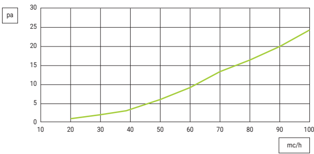
ATTACCHI LATERALI | SIDE SPIGOTS
